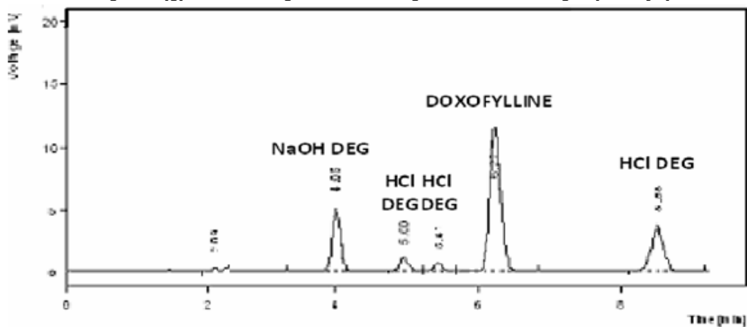
Figure 4(h): Chromatogram - Mixture of Doxofylline Degradation Products Figure 4(a-h): Results of various forced degradation study
