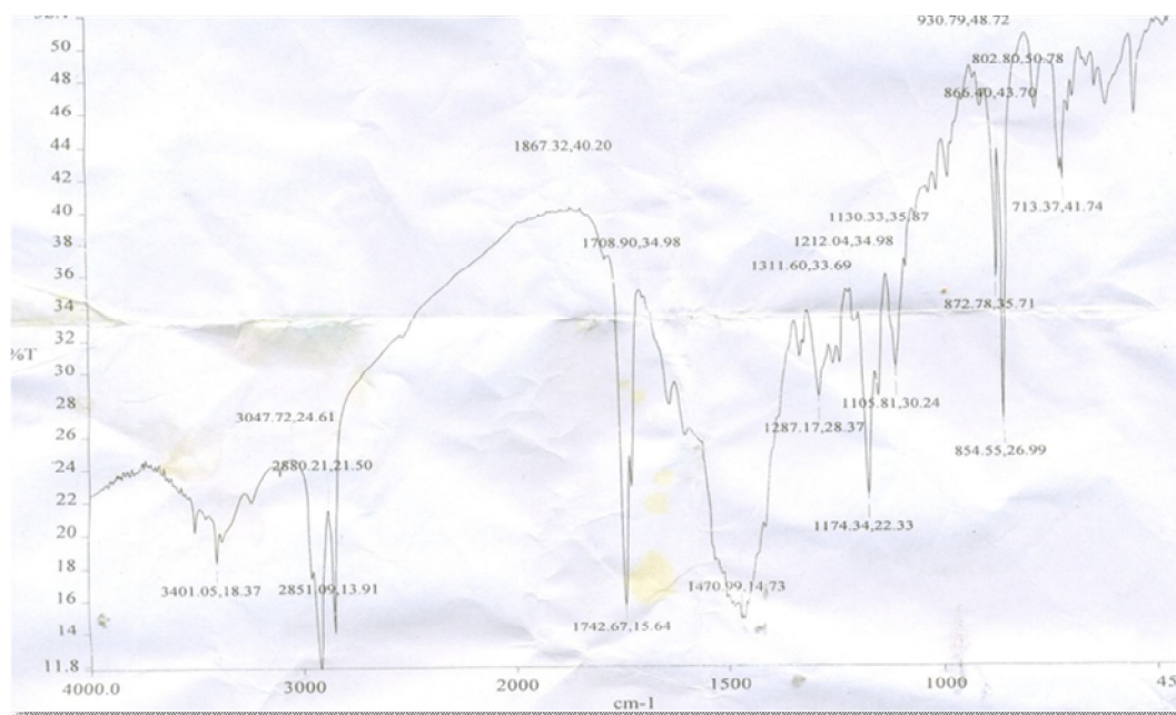
Figure 13: FTIR spectra of physical mixture of chitosan based formulation
