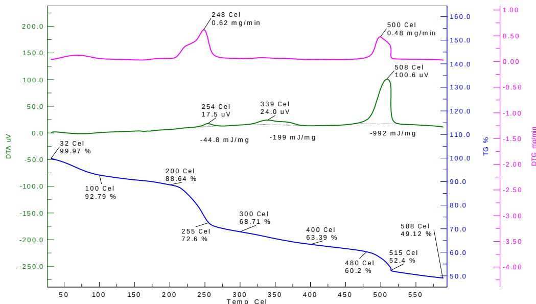
Figure 7: Thermogram of physical mixture of Chitosan based formulation
