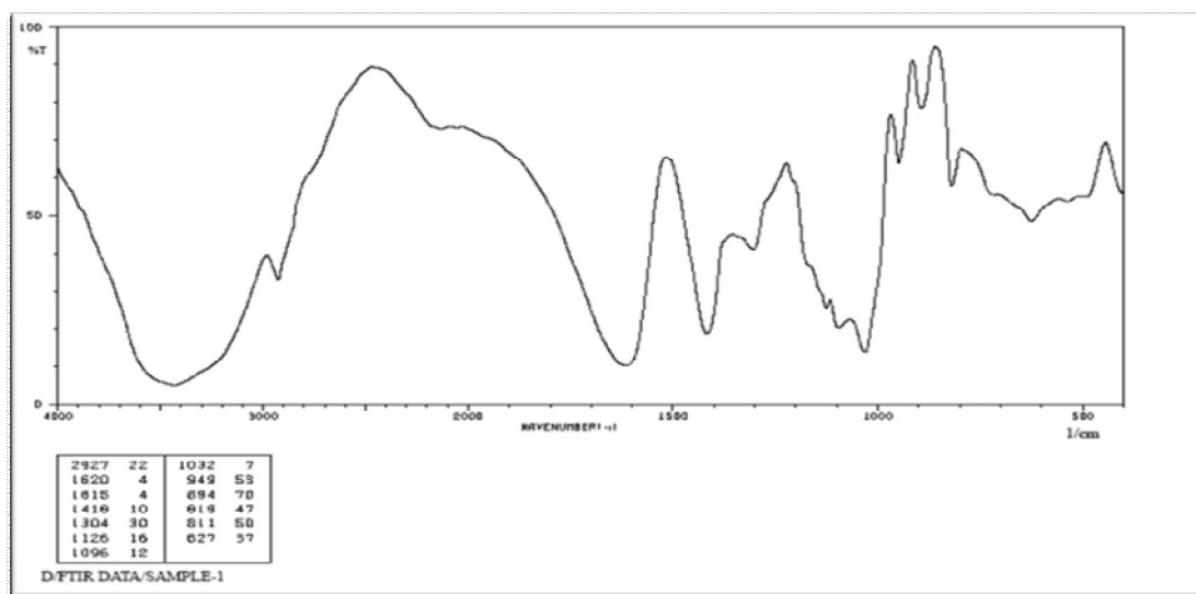
Figure 9: FTIR of Sodium Alginate
