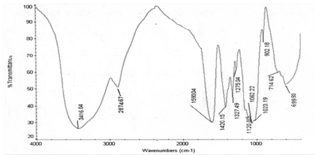
Figure 10: FTIR of Chitosan
