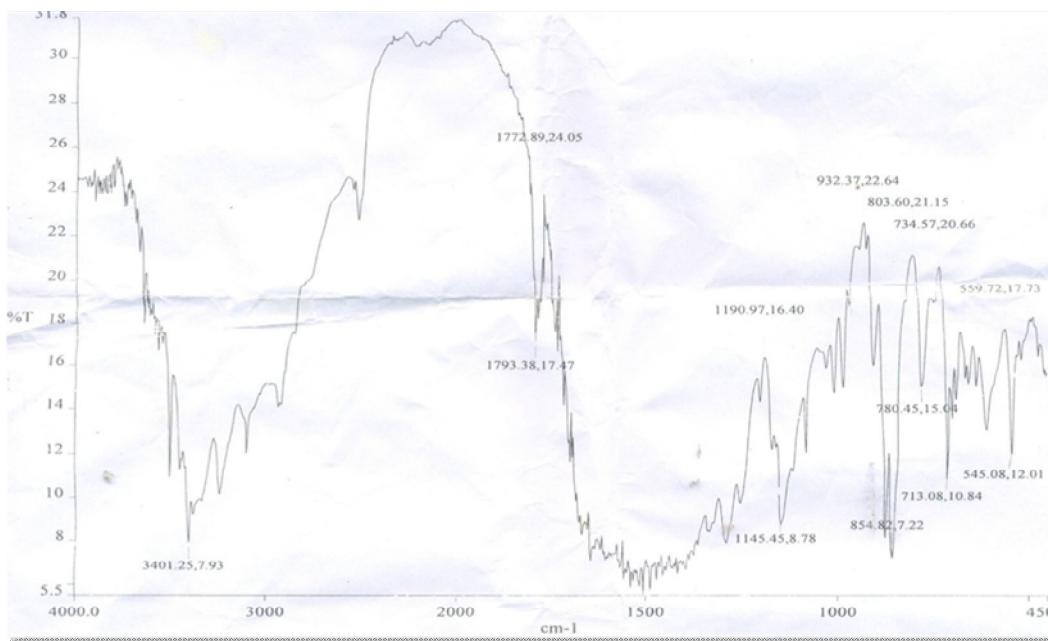
Figure12: FTIR spectra of physical mixture of sodium alginate based formulation
