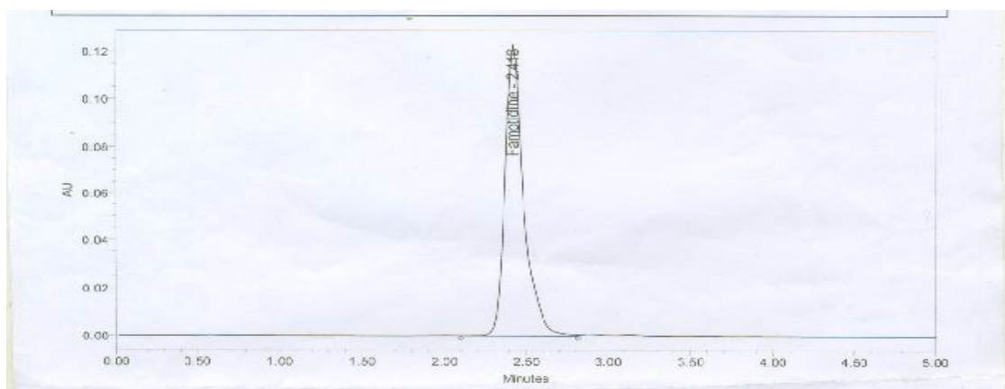
Figure 1: Chromatogram of Famotidine
