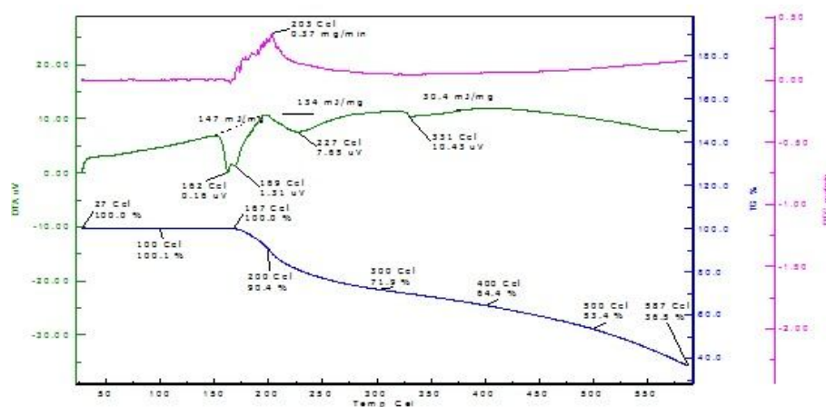
Figure 2: Thermogram of Famotidine
