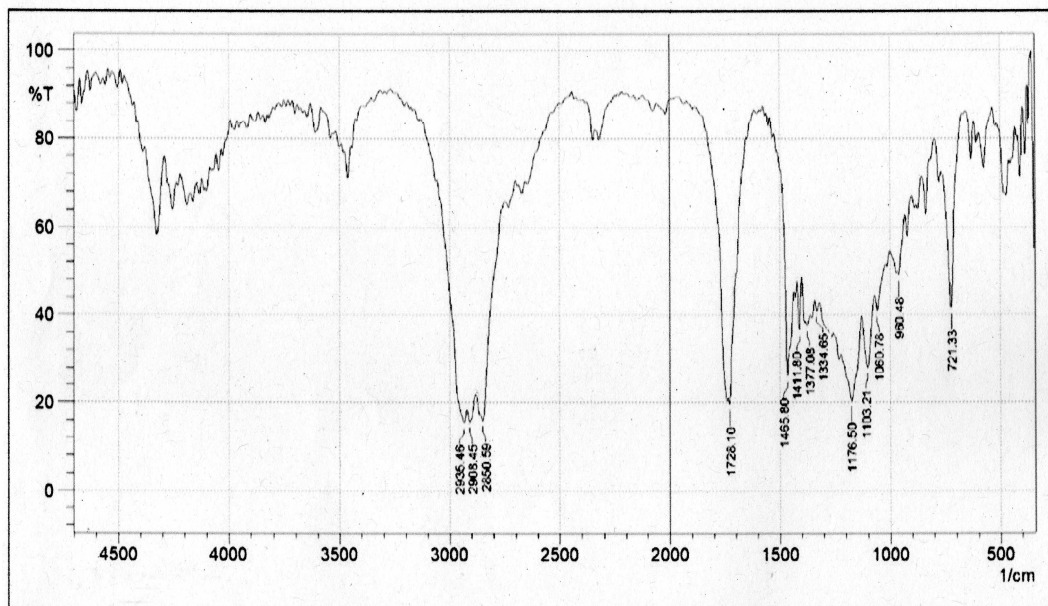
Figure 11: FTIR of Gelucire 43/01
